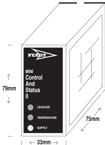
MiniCAS II supervision relay
