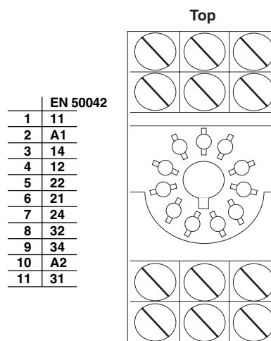
11 pin relay base
